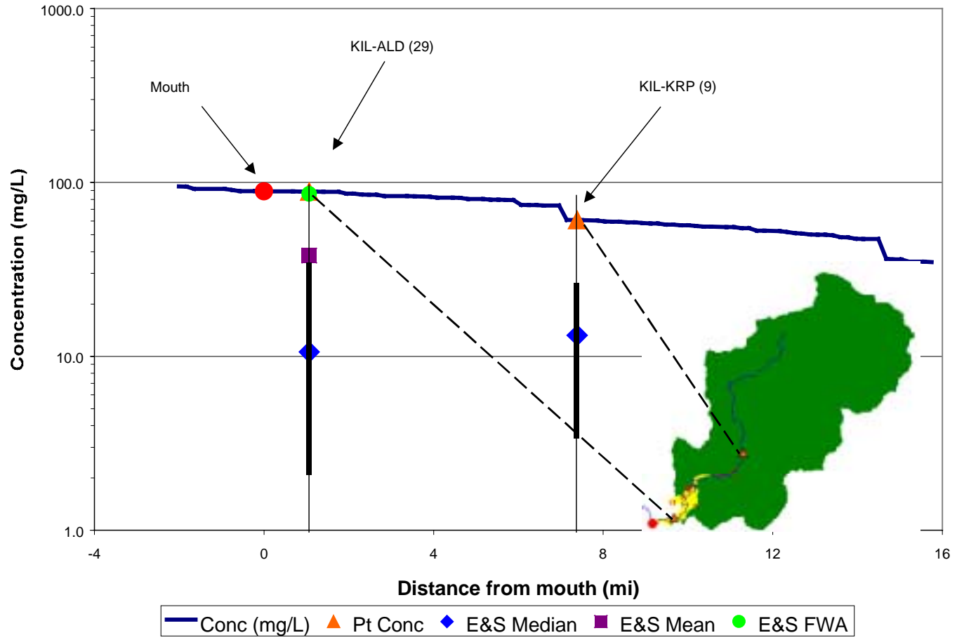
Figure 4-18. Kilchis River Sediment Concentration Profile Compared to Monitoring Data
