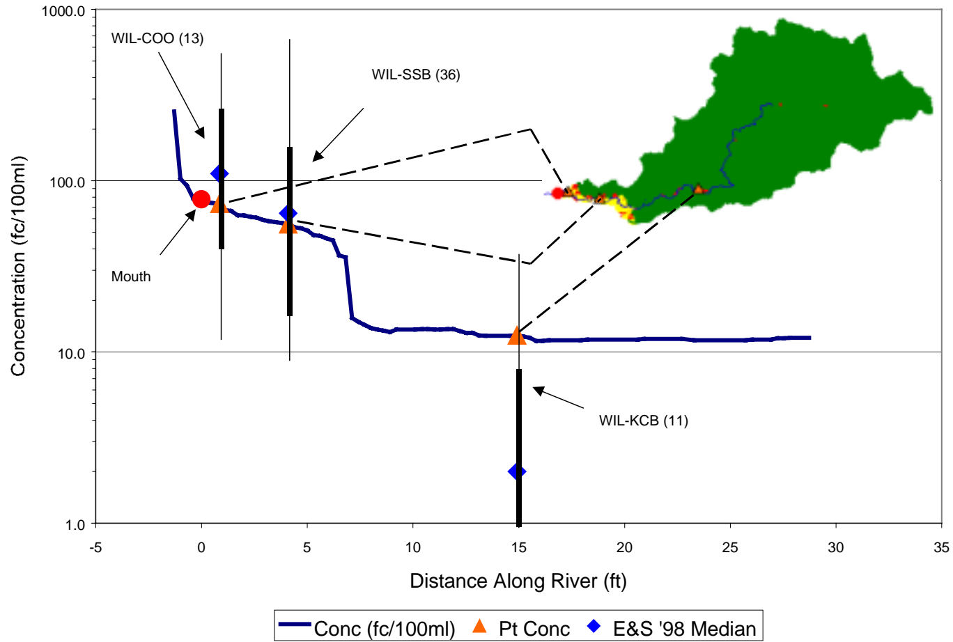
Figure 4-12. Wilson River Bacteria Concentration Profile Compared to Monitoring Data
