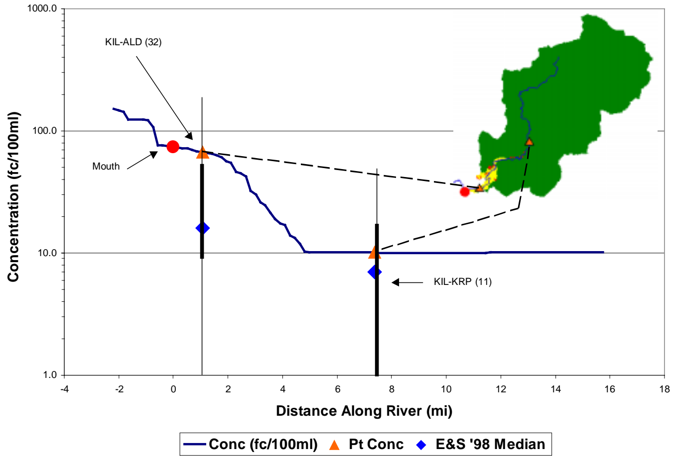
Figure 4-11. Kilchis River Bacteria Concentration Profile Compared to Monitoring Data
