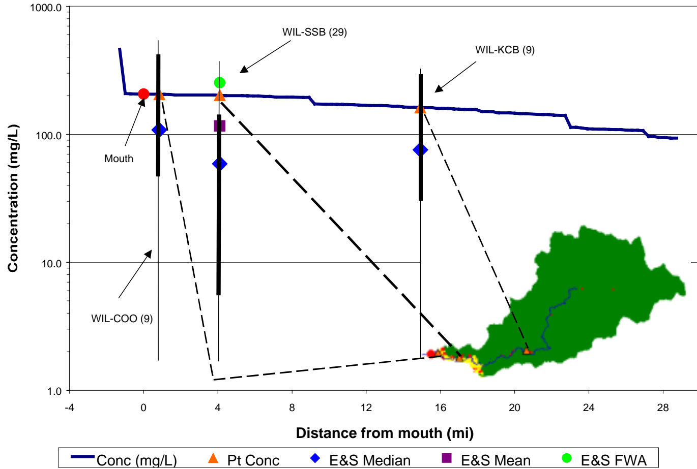
Figure 4-19. Wilson River Sediment Concentration Profile Compared to Monitoring Data
