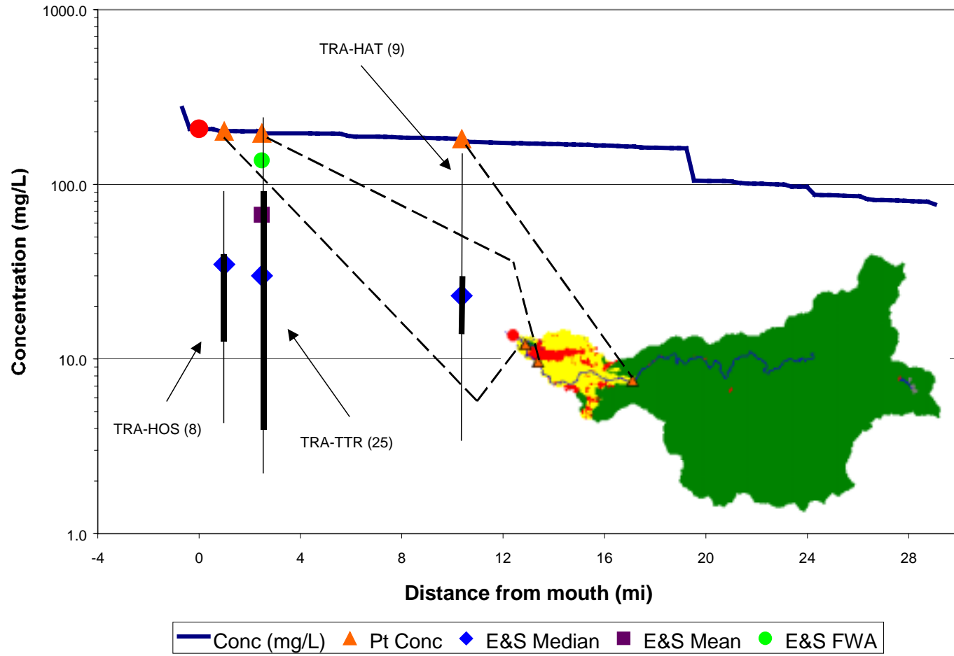
Figure 4-20. Trask River Sediment Concentration Profile Compared to Monitoring Data
