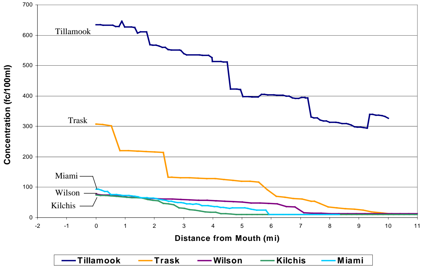
Figure 4-15. Comparison of Bacteria Concentration Profiles for the Five Rivers in the Watershed
