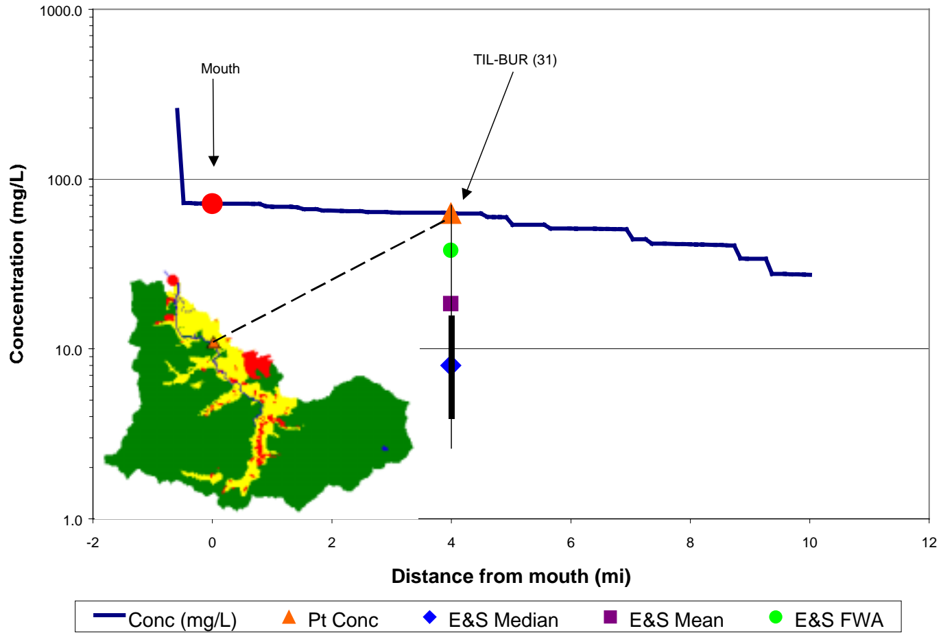
Figure 4-21. Tillamook River Sediment Concentration Profile Compared to Monitoring Data
