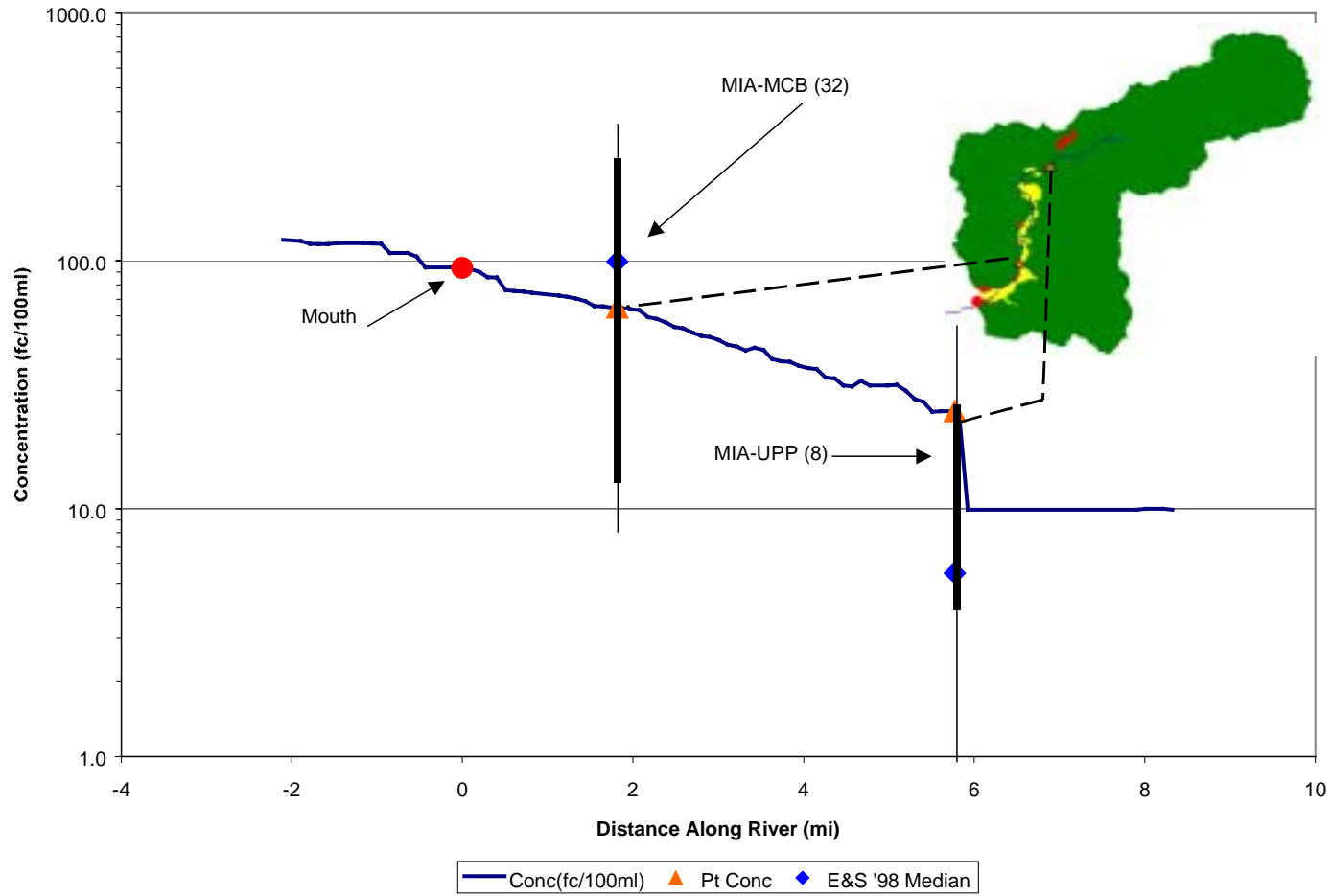
Figure 4-10. Miami River Bacteria Concentration Profile Compared to Monitoring Data
