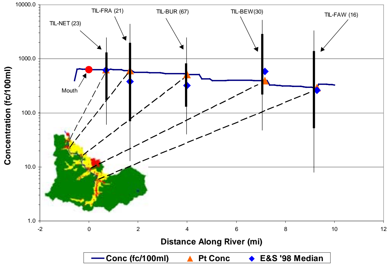
Figure 4-14. Tillamook River Bacteria Concentration Profile Compared to Monitoring Data
