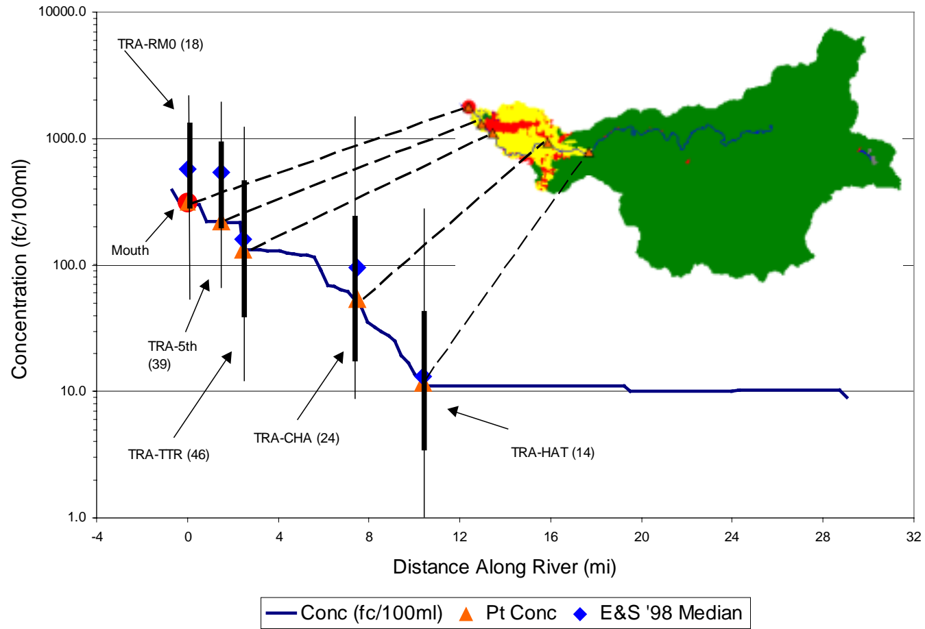
Figure 4-13. Trask River Bacteria Concentration Profile Compared to Monitoring Data
