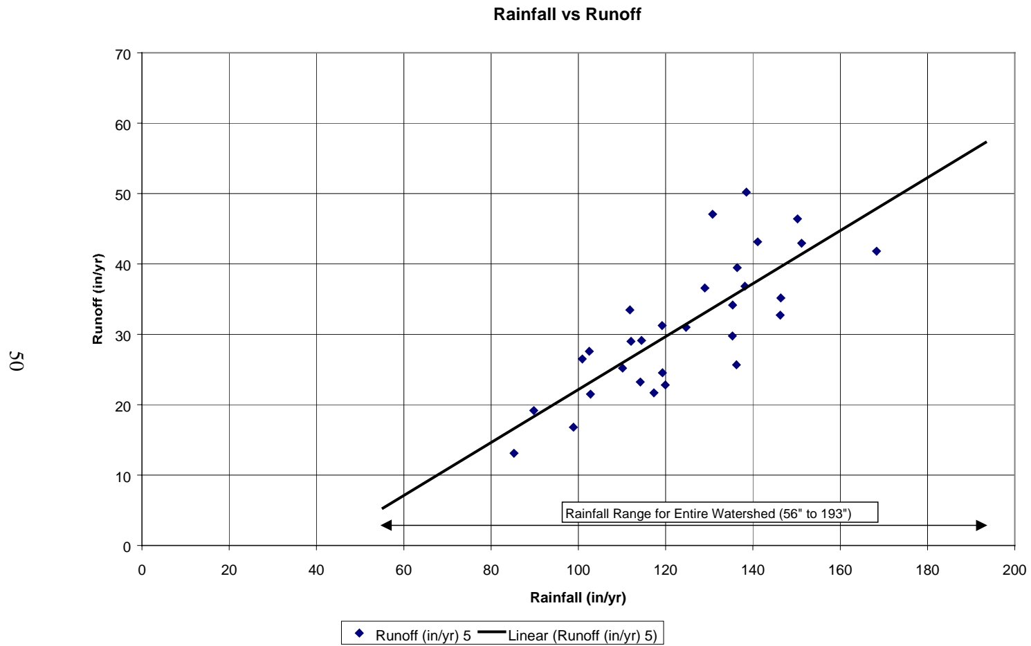
Figure 3-13. Graph of Annual Rainfall versus Annual Runoff For the Wilson River
