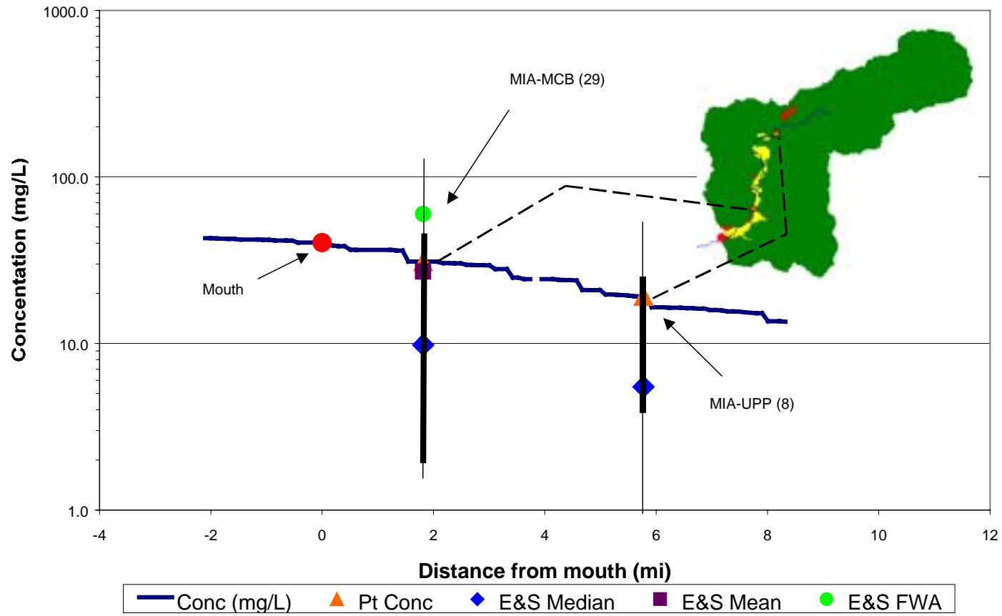
Figure 4-17. Miami River Sediment Concentration Profile Compared to Monitoring Data
